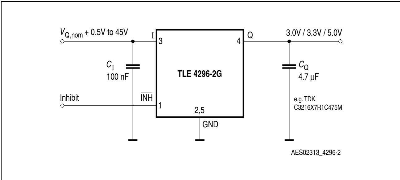
Figure 3 Application Circuit
